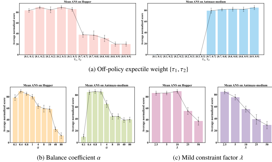
Fig. G.2. Decision-making quality of ISSP under varying off-policy expectile regression weight \{\tau_1, \tau_2\} , balance coefficient \alpha , and mild constraint factor \lambda , on the Hopper and Antmaze-medium environments.
