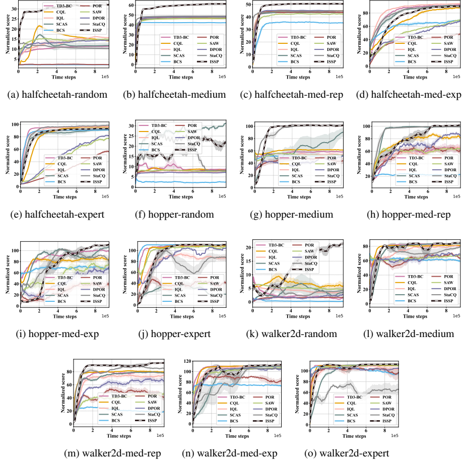
Fig. H.3. Normalized score learning curves of ISSP against ORL baselines on the D4RL MuJoCo dataset tasks. The centerline and its shadow represent the mean and standard deviation across five seeds, respectively. Smoothing via a moving average window is applied to enhance visual clarity. medium-replay=med-rep, medium-expert=med-exp
